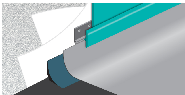
5. Floor Trim Detail
