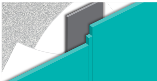
3. Welded Joint Detail
